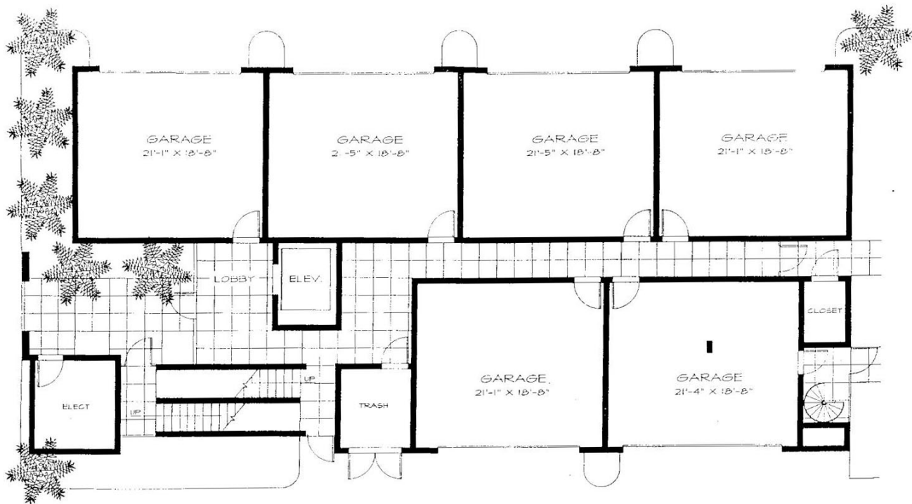
Sun Harbour Club First Level Floor Plan www.buymarco.com
