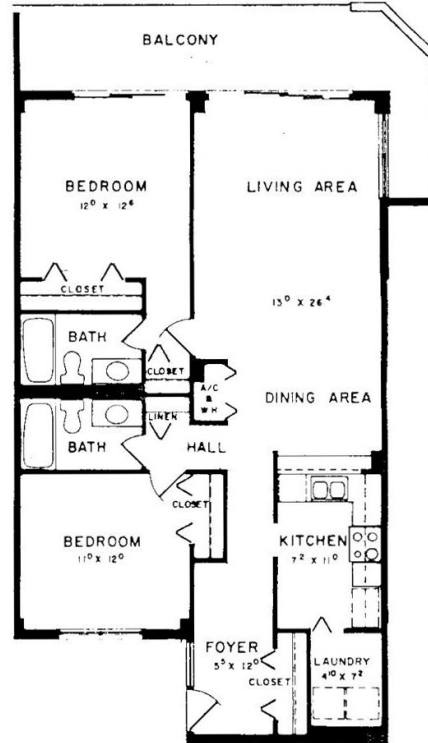
APARTMENTS 201, 301, 401, 501, 601 - AS SHOWN 207, 307, 407, 507, 607 - REVERSE
