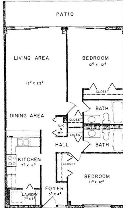
APARTMENT 106 - AS SHOWN APARTMENT 112 - REVERSE
