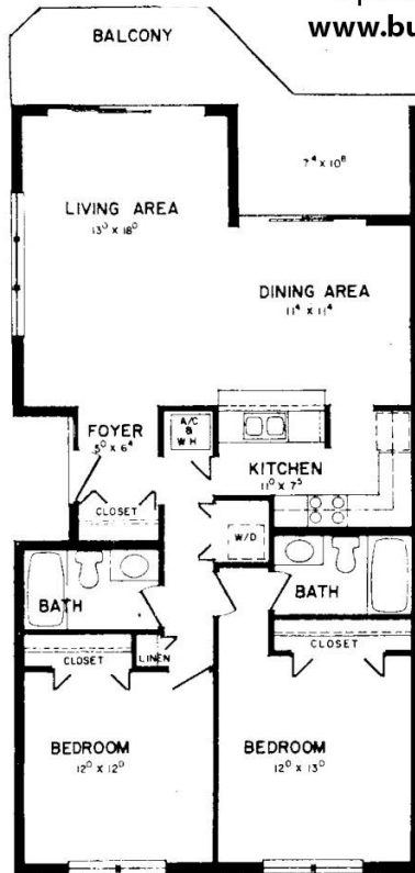
APARTMENT 3 - BUILDINGS E, G, J, L, P, R - AS SHOWN APARTMENT 4 - BUILDINGS D, F, H, K, M, Q - REVERSE
